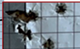
Yaw measurements indicate barrel has reached failure level for MIL-B-11595.
